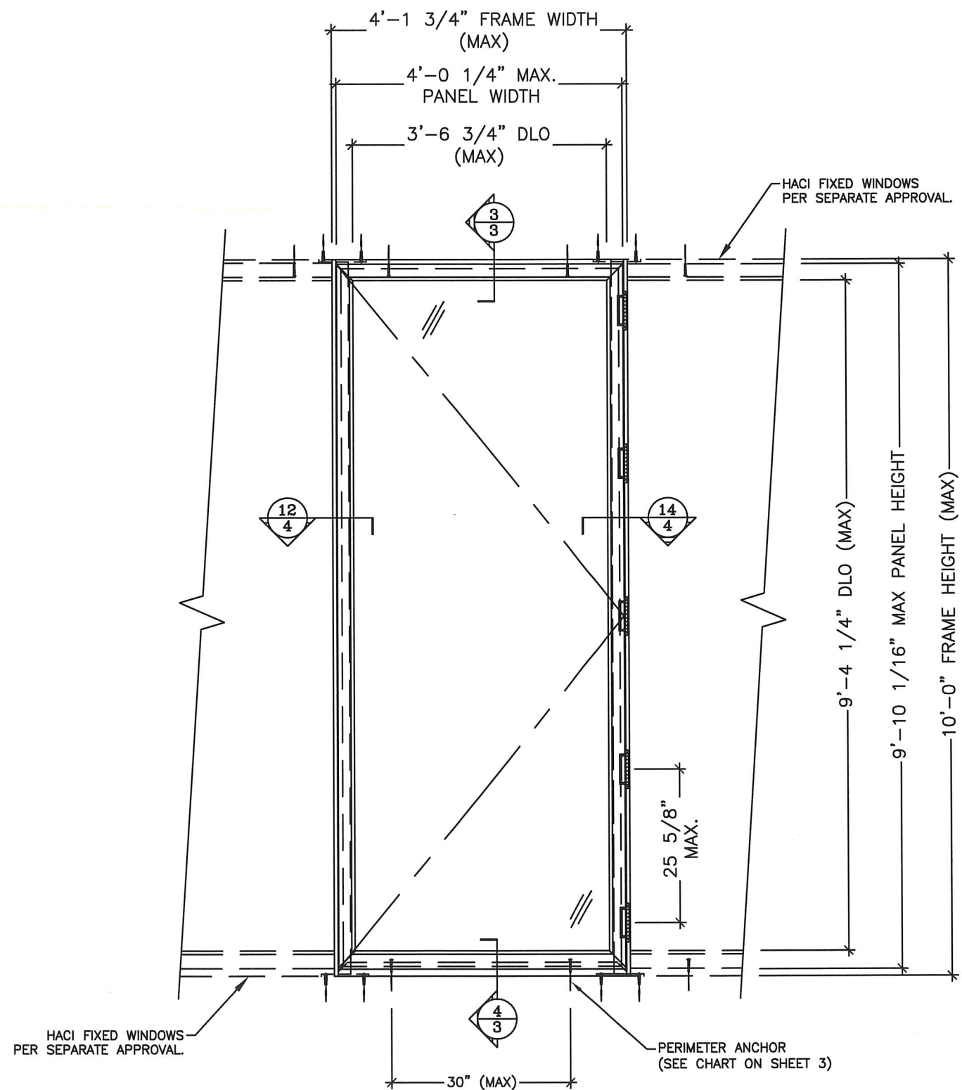
② SINGLE OUTSWING DOOR MULLED WITH FIXED WINDOWS (EXTERIOR VIEW)
