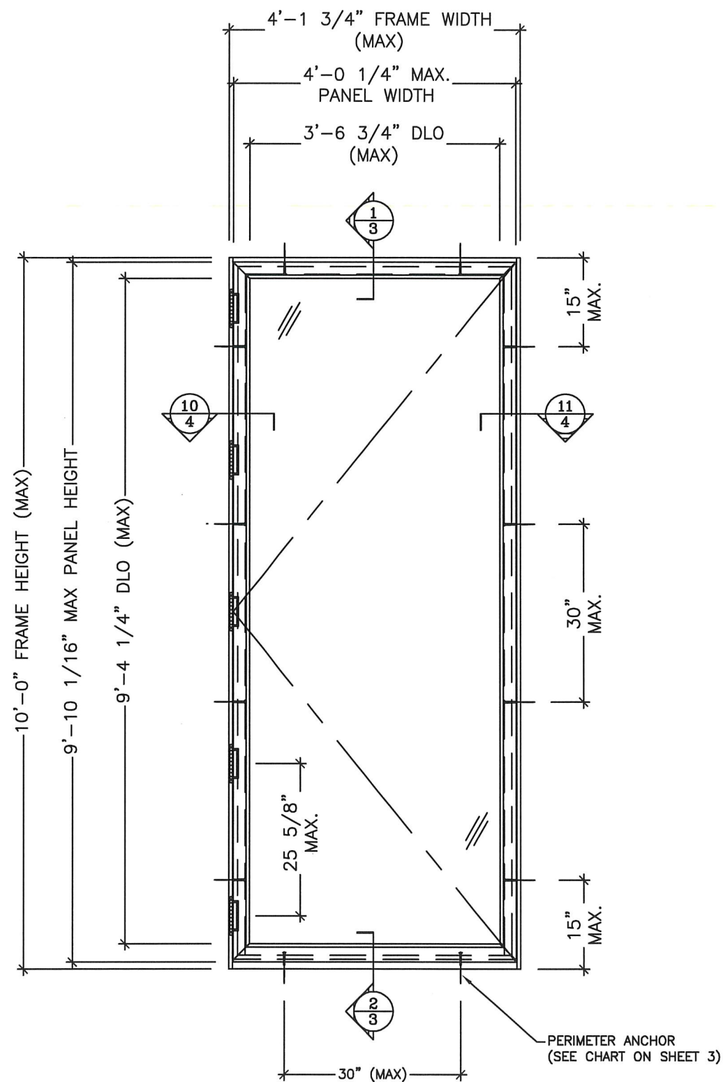
① SINGLE OUTSWING DOOR (EXTERIOR VIEW)
